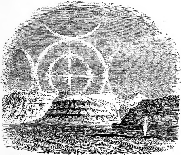
MOCK SUNS.
